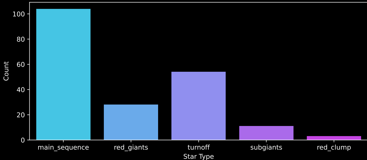
APOGEE DR17 Field: [184-43_MGA] Count plot of Star Type
