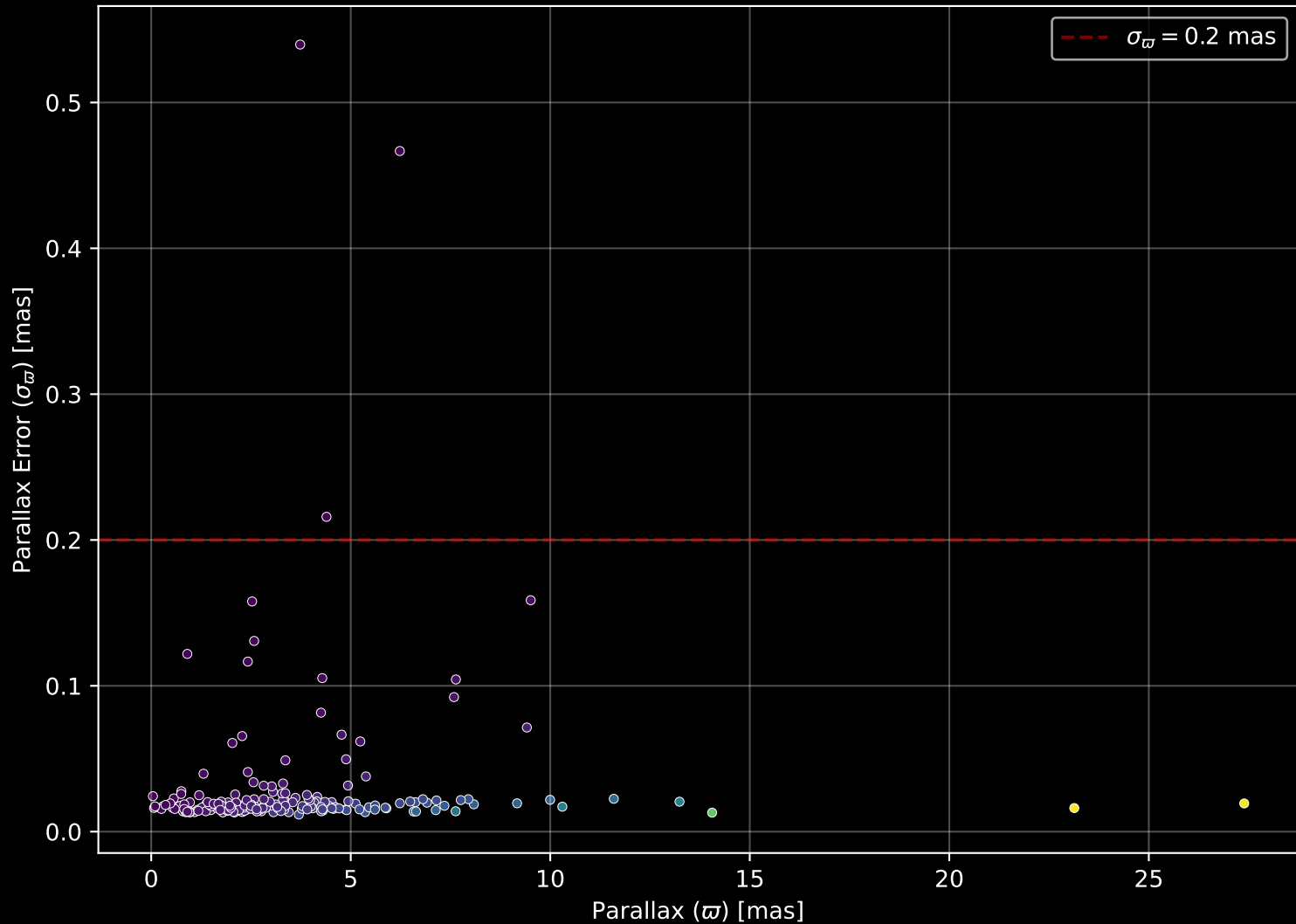
APOGEE DR17 Field: [184-43_MGA] Parallax Quality (n= 200)
