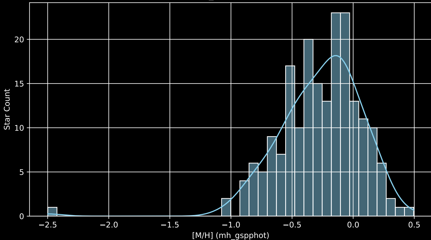
APOGEE DR17 Field: [184-43_MGA [M/H] (mh_gspphot) (n= 199)
