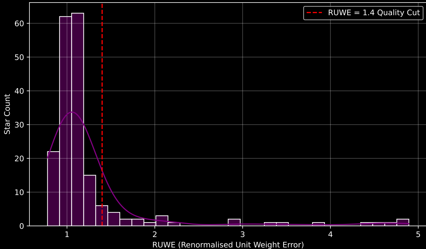
GAPOGEE DR17 Field [184-43_MGA] RUWE Distribution (n= 191)
