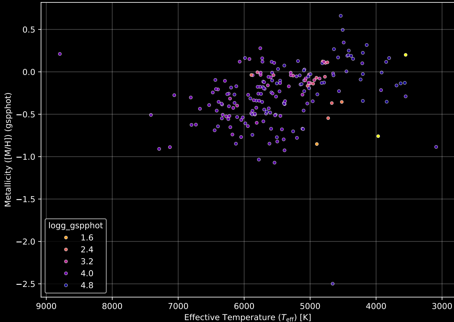
APOGEE DR17 Field: [184-43_MGA] Stellar Population Parameters (n= 200)
