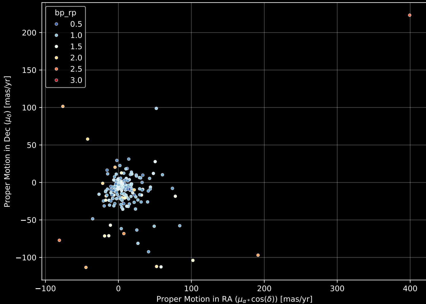
APOGEE DR17 Field: [184-43_MGA] Proper Motion Diagram (n= 200)
