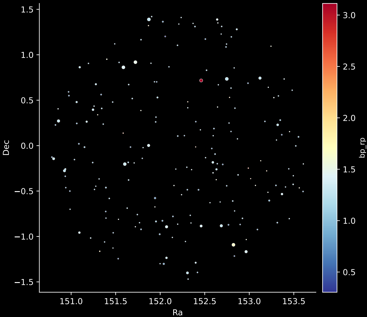
APOGEE DR17 Field: [184-43_MGA] Stars: 200
